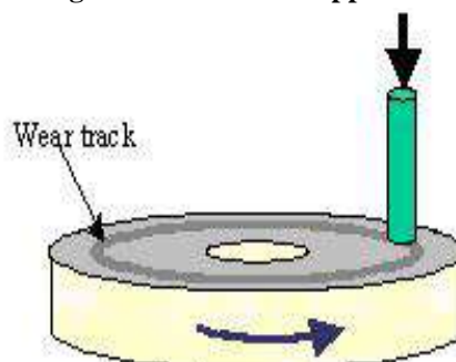
Figure 4: Pin-on-disc apparatus
