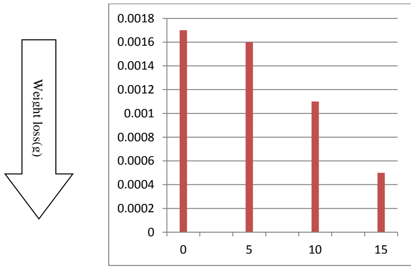
Graph.2. Effect of Filler % on wear rate.
