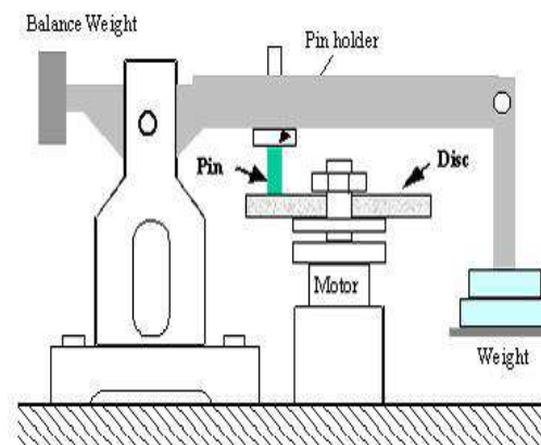
Figure 4: Pin-on-disc apparatus
