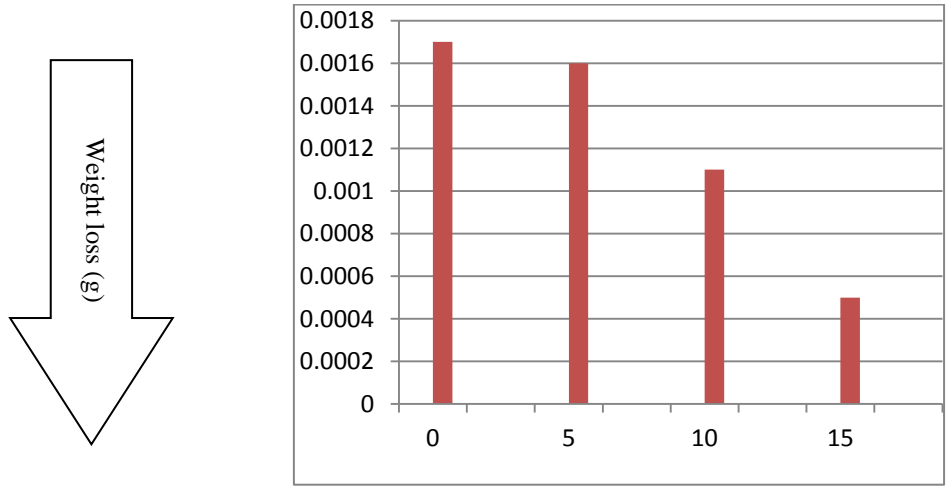
Graph.1. Variation of wear for different Filler % (by weight)
