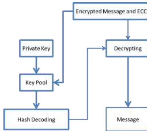
Figure3: Decryption phase
