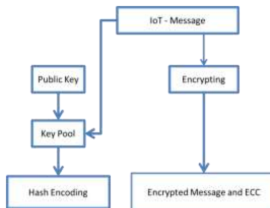
Figure2: Encryption phase
