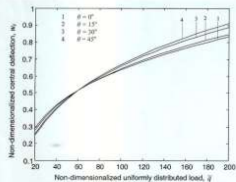
Fig. 6 Variation of central deflection with pressure of simply supported (SS4) anti-symmetric square plate of the arrangement [0^{\circ}/\theta^{\circ}/\theta^{\circ}/0^{\circ}] with different orientations ( h/a = 0.2 ).
