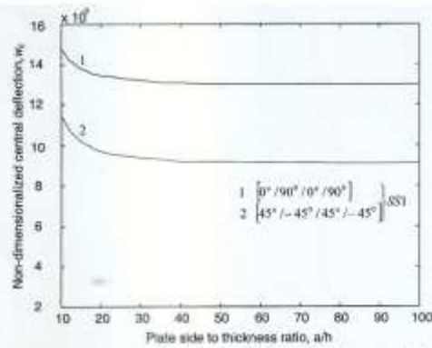
Fig. 2 A comparison of the non-dimensionalized centre deflections versus side to thickness ratio of anti-symmetric cross-ply and angle-ply square laminates under uniform lateral load ( \bar{q} = 1.0 ).
