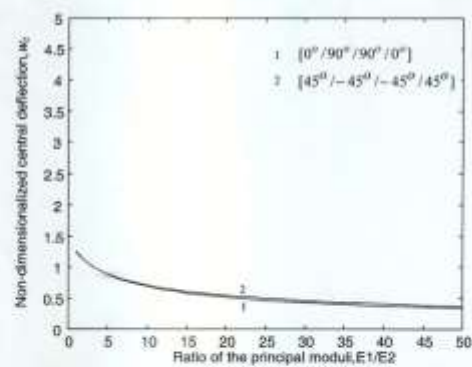
Fig. 4 Effect of material anisotropy on the non-dimensionalized centre deflections of a four layered symmetric cross-ply and angle-ply simply supported laminates (SSS) under uniform lateral load ( \bar{q} = 100.0 , h/a = 0.1 ).
