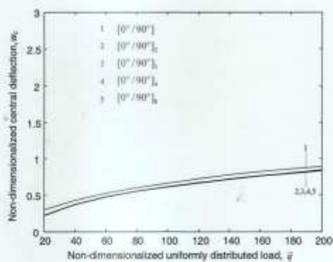
Fig. 3 Number of layers effect on a simply supported (SSS) anti-symmetric cross-ply [0^{\circ}/90^{\circ}]_n square plate under uniformly distributed loads ( h/a = 0.1 ).
