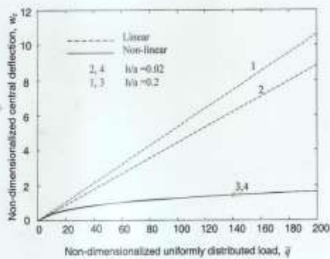
Fig. 1 Variation of central deflection with load of thin and thick simply supported (SSS) square isotropic plate.
