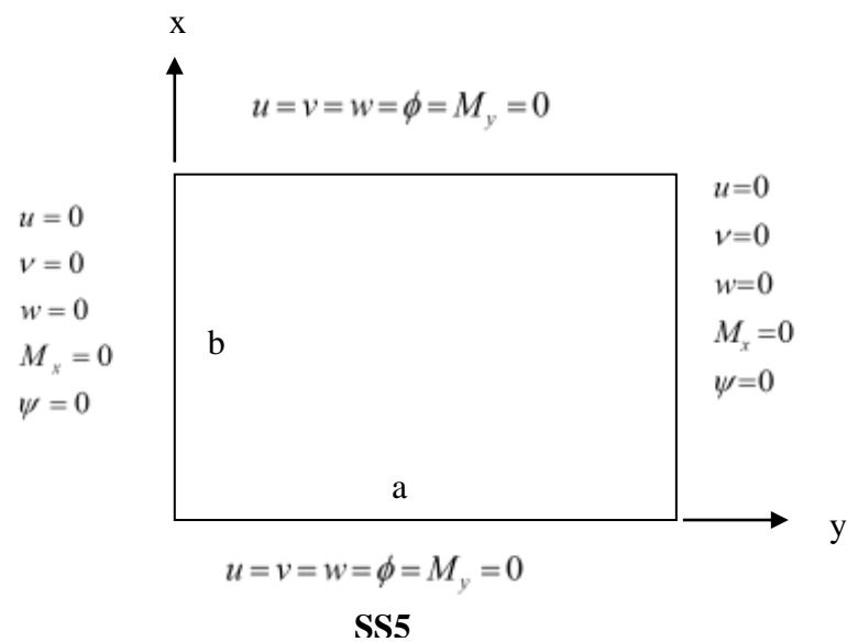
Fig. (1) Simply supported boundary condition
